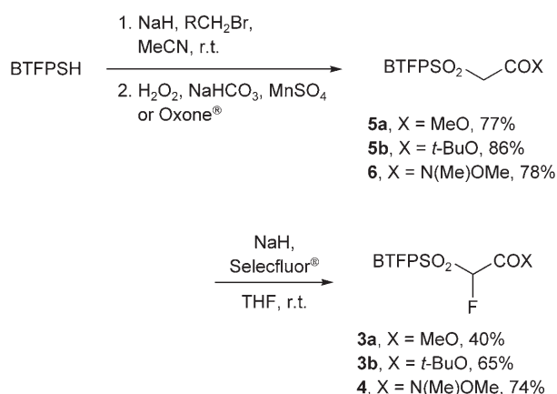
Scheme 1. Synthesis of fluorinated BTFP sulfones 3 and 4 .
