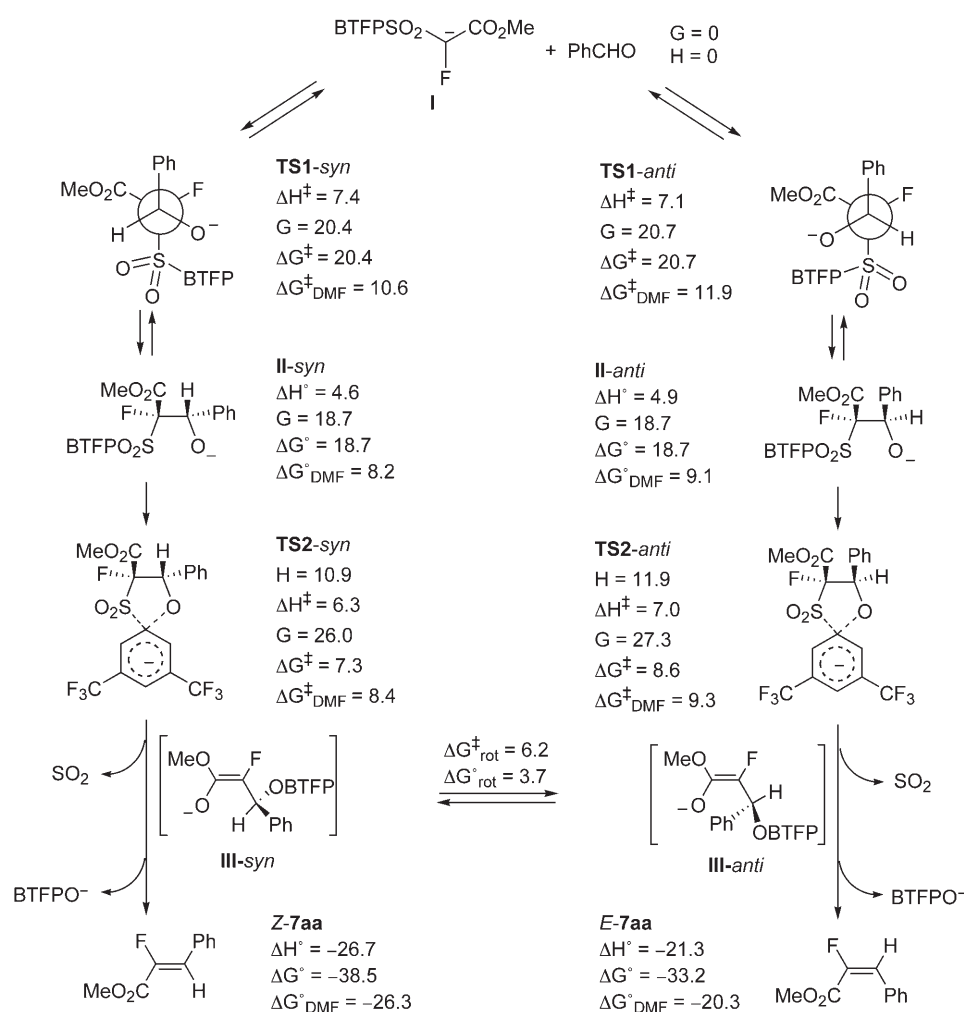
Scheme 2. Proposed mechanism for the fluoro-Julia-Kocienski olefination of aldehydes with BTFP sulfones.
