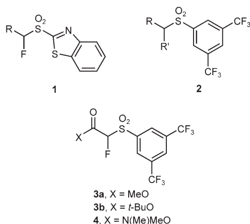
Figure 1. BT and BTFP sulfones 1–4 .
