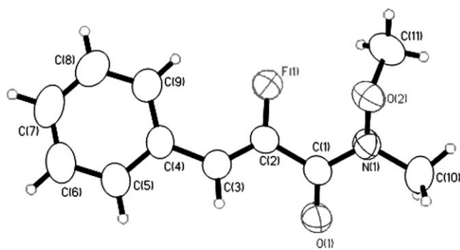
Figure 2. X-ray structure of 9a .
