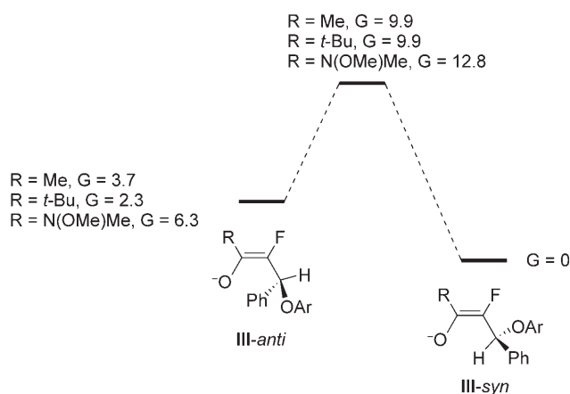
Figure 3. Rotation energies (kcal mol -1 ) for intermediates III for BTFP sulfones 3 and 4 .
